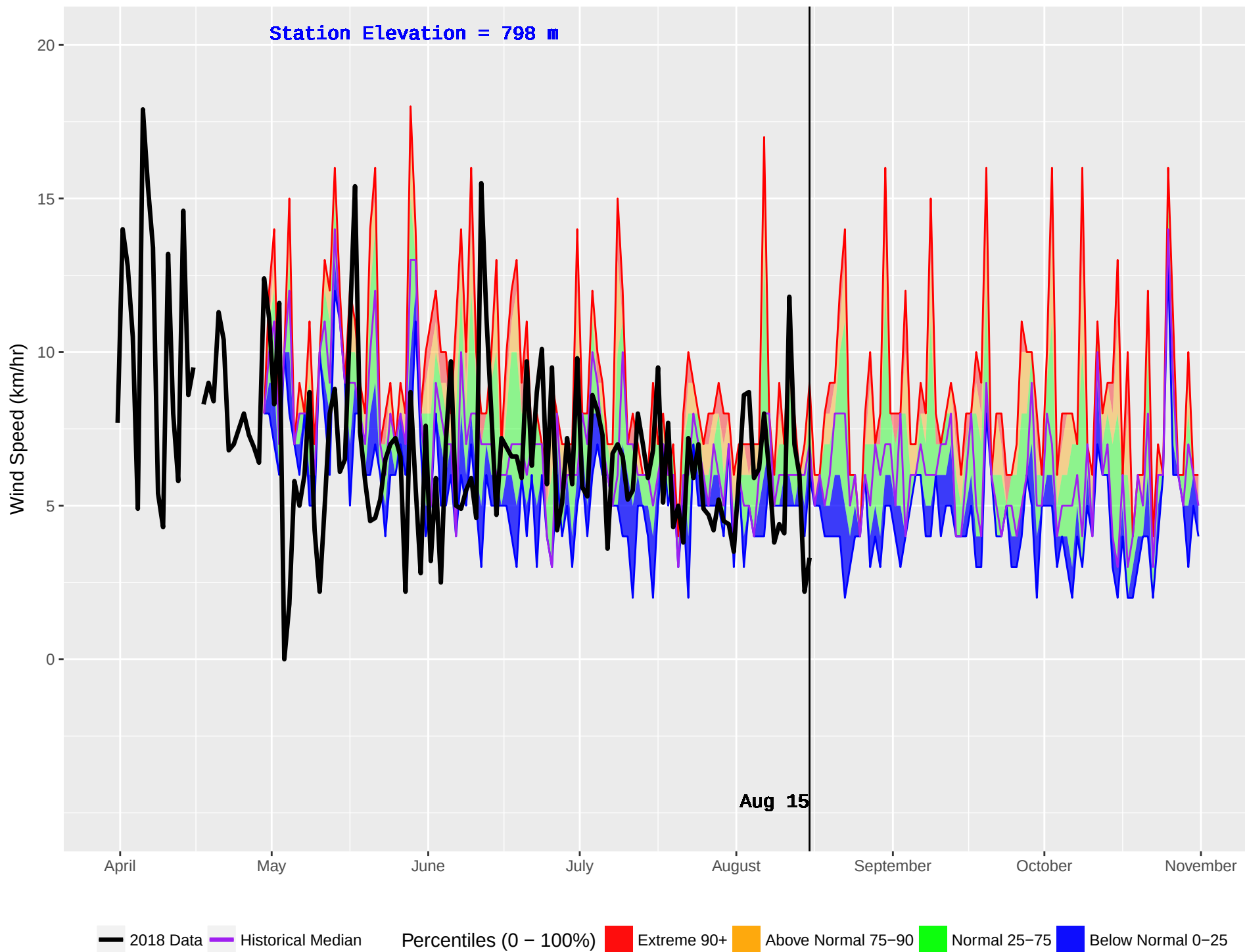
SEVEREID (1165) : Historical (2014–2016) and Current (2018) Daily Wind Speed
